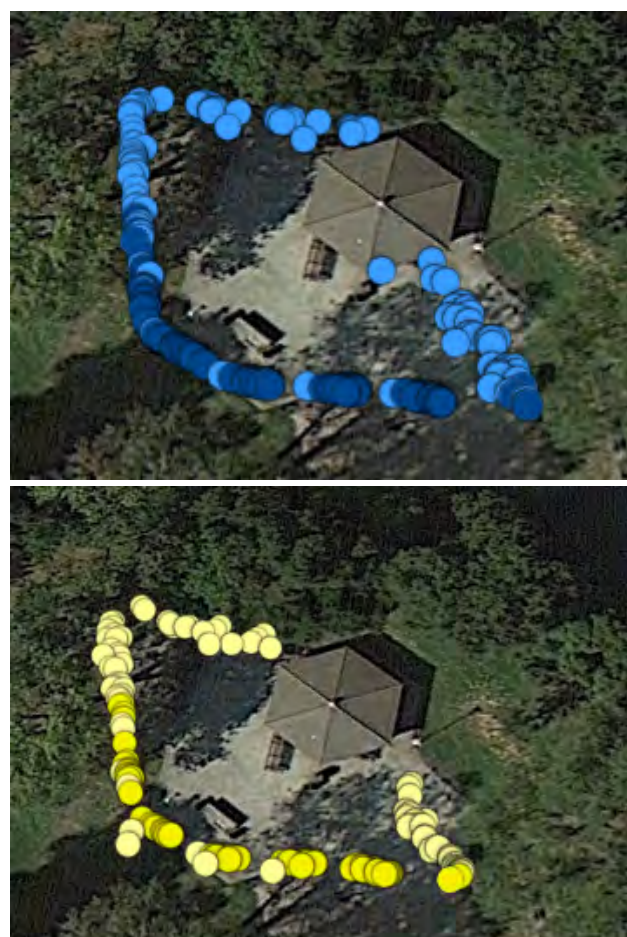
Figure 9: Fixed RTK and float positions – ProMark 220 in blue (top) and competitive product in yellow (bottom), when a competitive brand base is used.
